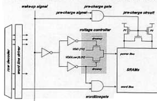
FIGURE 7. Implementation of the drowsy cache line
