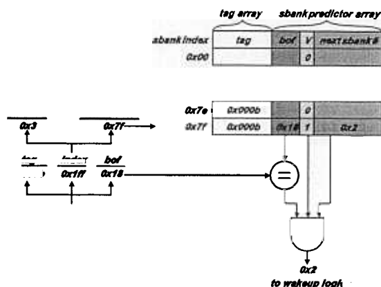
FIGURE 10. Next sub-bank predictors in cache tags
