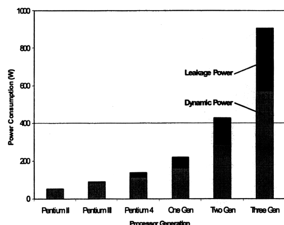
FIGURE 1. Dynamic and static power trends
