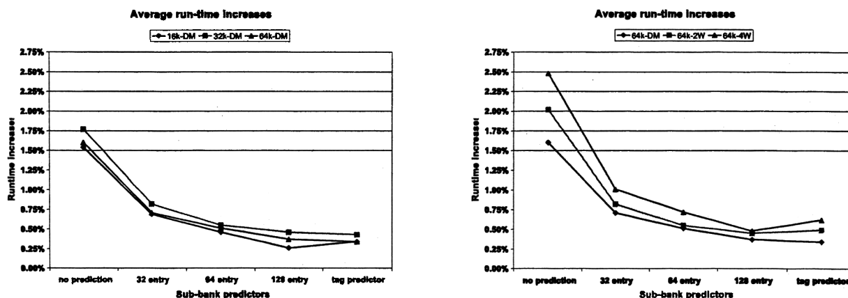
FIGURE 13. Average run-time increases of various sub-bank predictors.
