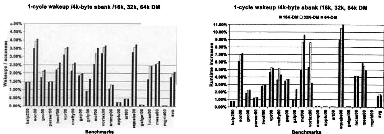
FIGURE 3. Wake-up overhead and run-time increase
