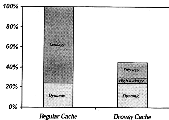
FIGURE 2. Energy reduction using the drowsy cache
