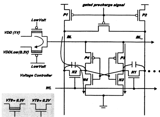
FIGURE 11. Implementation of a drowsy memory cell.
